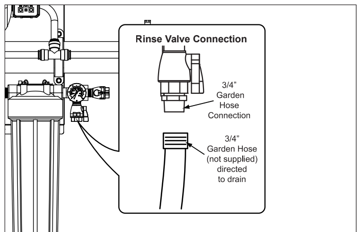
Figure 2. Rinse Valve Connection
