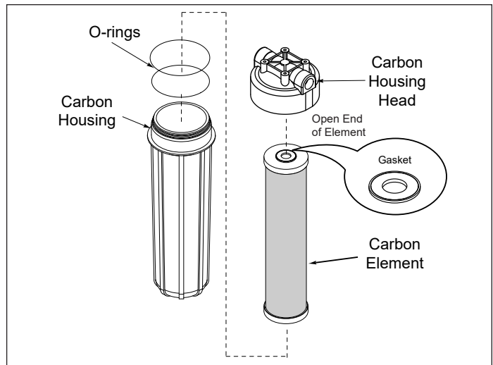
Figure 1. Replacing the Carbon Element
