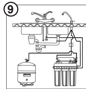
Make tubing connections.
