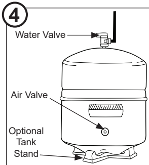
Attach tank valve and mount tank.
