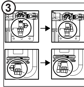
Open RINSE valve and open INLET valve
