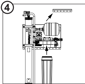
Hang system and install empty carbon bowl.
